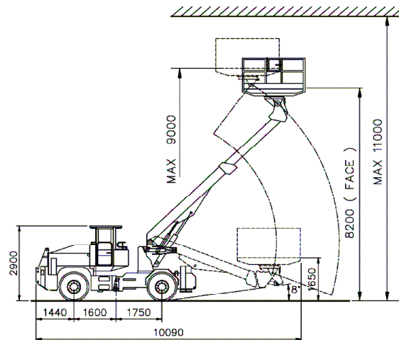
Himec 9910 B Rex – 1000 kg
