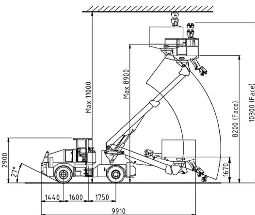
Himec 9915 BA – 1500 kg
