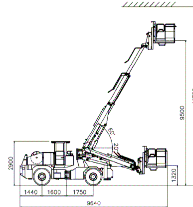
Himec 9905 BT – 2 x 500 kg
